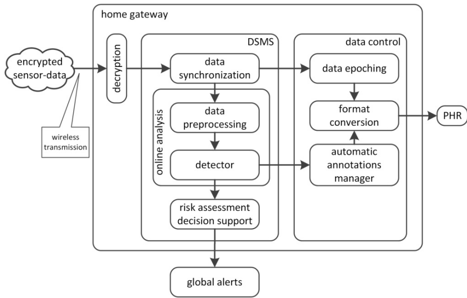
Fig.2: Block diagram of the multimodal streaming data processing architecture.
