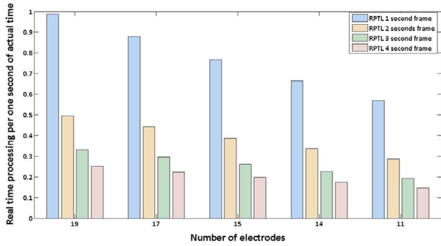
2 Fig. 7. Real time processing corresponding to each second of actual time, for various frame sizes and 3 number of electrodes.
