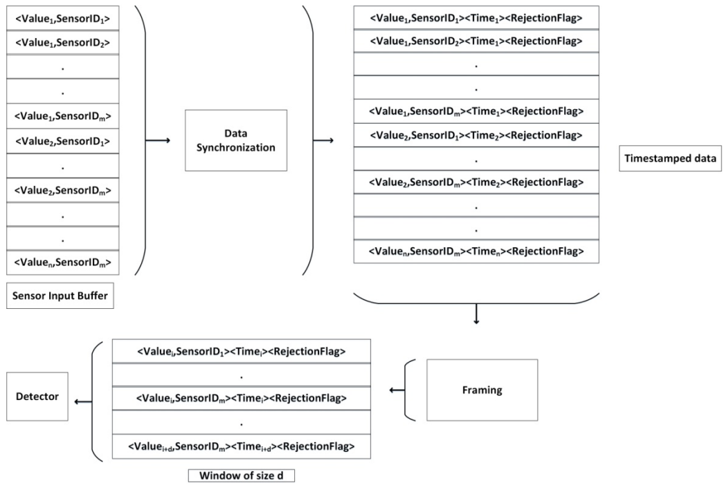
Fig. 5: Synchronization and processing data flow.
