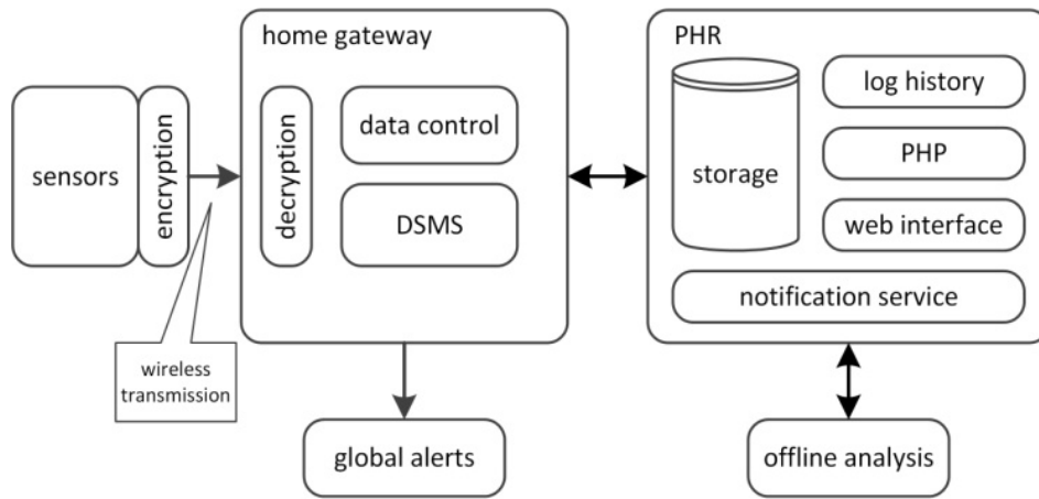
Fig. 1: Block diagram of the ARMOR's concept.
